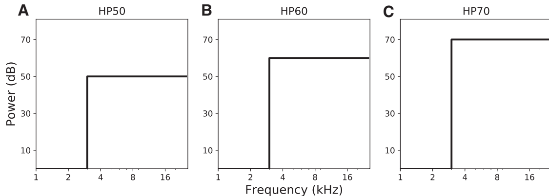
Figure 1. Schematized power spectra of the sound stimuli used in the pre-adaptation/post-adaptation experiment. Stimuli were derived from a GWN control stimulus by removing all frequencies below 3 kHz (HP), at (A) 50-dB SPL (A-weighted), (B) 60 dBA, or (C) 70 dBA.
