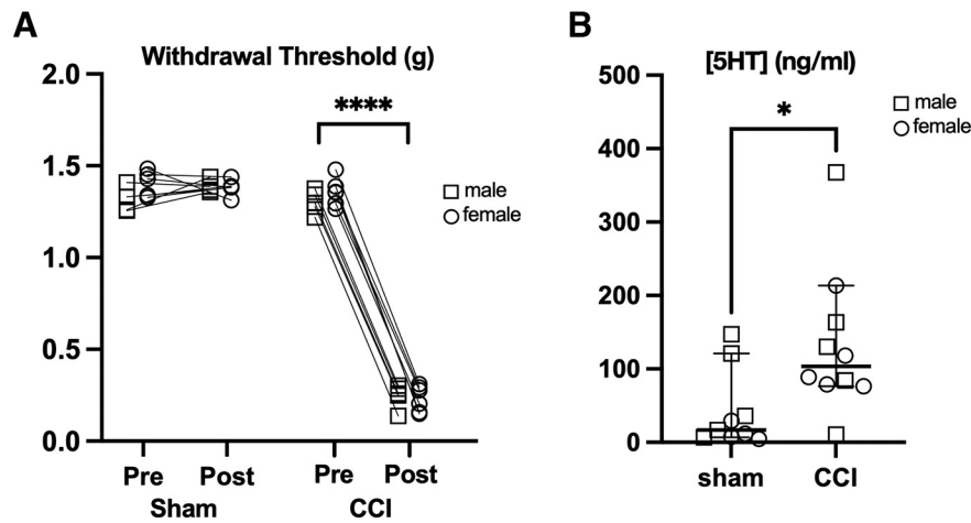
Figure 3. Tonic serotonin levels are elevated in SpVc in a mouse model of neuropathic pain. A , CCI-ION reduces withdrawal thresholds to mechanical stimulation of the orofacial region. B , Concentrations of serotonin in isolated SpVc tissue were quantified by liquid chromatography-tandem mass spectrometry (LC-MS/MS). Group sizes: n = 9 sham and n = 11 CCI, p = 0.018 , unpaired t test. *p < 0.05 , ****p < 0.0001 .
