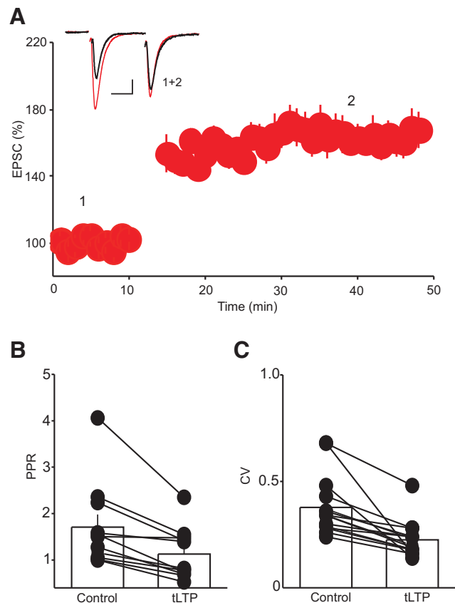
Figure 2. Decrease in PPR and CV indicate a presynaptic expression of tLTP. A , Summary graph of tLTP assessed using pairs of stimuli. B , Histogram summary of the average PPR ( EPSC_2/EPSC_1 ) obtained before and during the tLTP. Inset depicts superimposed EPSC traces evoked by paired-pulse stimulation taken at the time point indicated by number. Scale bars: 50 pA, 20 ms. C , Histogram summary of the average CV obtained before and during the tLTP. Note that the tLTP is associated with a significant decrease in PPR (*, p < 0.05 , n = 11 ) and CV (*, p < 0.05 , n = 15 ).
