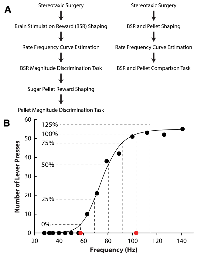
Figure 1. Experimental overview and sample BSR selection. A , Two groups of rats were tested, 13 in the first group (left) and five in the second (right). B , Sample rate–frequency curve and delineations of each reward used in the BSR tasks. Frequencies were selected for each animal based on percentages of the central linear portion of their sigmoidal rate–frequency curve.
